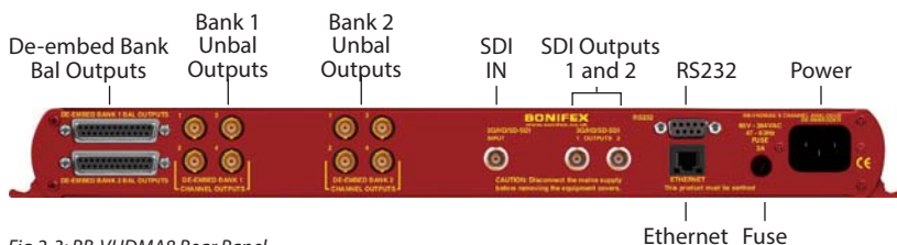
Fig 2-3: RB-VHDMA8 Rear Panel
