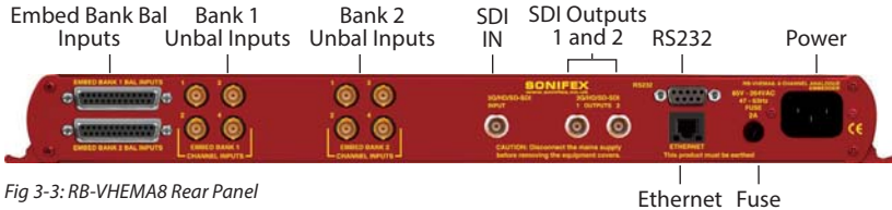
Fig 3-3: RB-VHEMA8 Rear Panel
