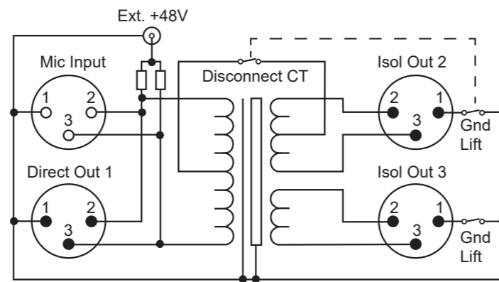
Fig 1-2: CM-MS3 Block Diagram
